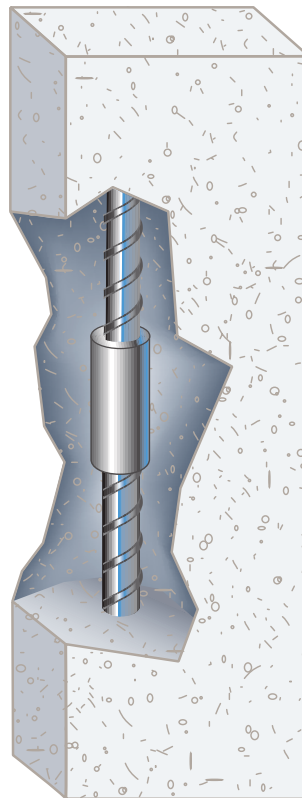
nVent LENTON mechanical couplers perform similar to a continuous length of rebar regardless of concrete condition.
